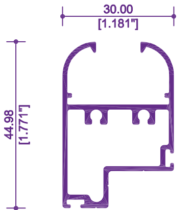
3503 / 12274 MARCO COLONIAL
