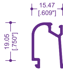
5085 / 12576 JUNQUILLO COLONIAL
